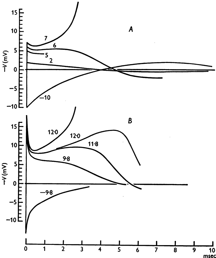
Fig. 21. A , numerical solutions of eqn. (26) for 6°C. The numbers attached to the curves give the initial depolarization in mV (also the quantity of charge applied in m\mu\text{coulomb/cm}^2 ). B , response of nerve membrane at 6°C to short shocks; the numbers show the charge applied in m\mu\text{coulomb/cm}^2 . The curves have been replotted from records taken at low amplification and a relatively high time-base speed.
