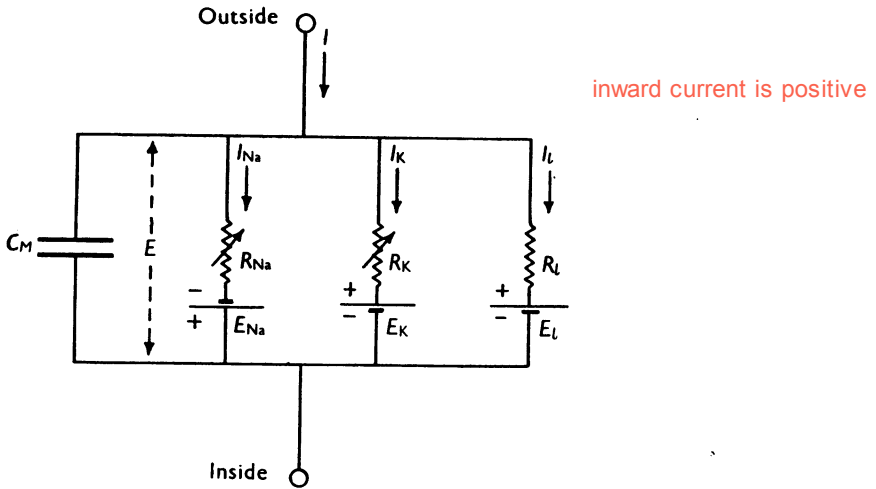
Fig. 1. Electrical circuit representing membrane. R_{Na} = 1/g_{Na} ; R_K = 1/g_K ; R_L = 1/\bar{g}_L . R_{Na} and R_K vary with time and membrane potential; the other components are constant.
